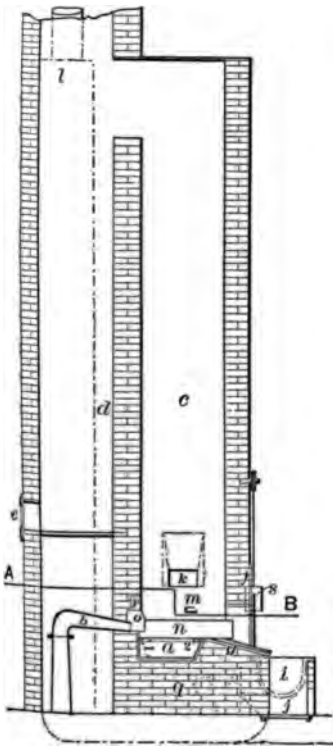
VERTICAL SECTION ON LINE C, D.
